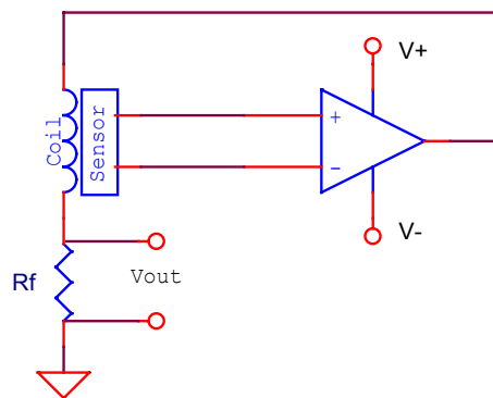
Fig. 4. Closed-loop magnetic field sensor.
