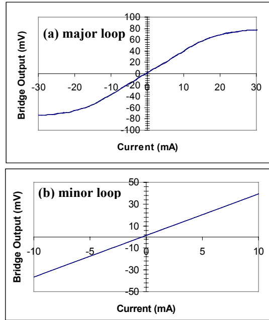
Fig. 7. Isolated bridge output to the signal current sweep in a fully processed analog isolator.
