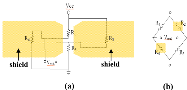
Fig. 2. Bridge sensor with flux concentrators: a) sensor configuration and b) Wheatstone bridge connection.
